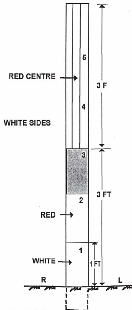
NO. 1 FLOOD GAUGE SIDE ELEVATION
